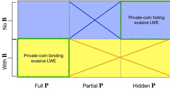
Figure 1: The above figure is adapted from [BUW24, Figure 1(b)] (BUW). BUW partition the private-coin evasive LWE based on whether \mathbf{B} is public or hidden (in both the pre- and post-conditions); and whether \mathbf{P} is public, hidden or “partially” hidden (in both the pre- and post-conditions). BUW then give simple counterexamples which rule out the different private-coin variants. Each counterexample is denoted by a cross of different color. Finally, the proposed classes of private-coin evasive LWE that survive their attack are indicated by the green outline. For simplicity of exposition, we do not mention an additional attack of BUW that allows the Samp algorithm takes \mathbf{B} as input, although we note that our attack subsumes that setting as well.
