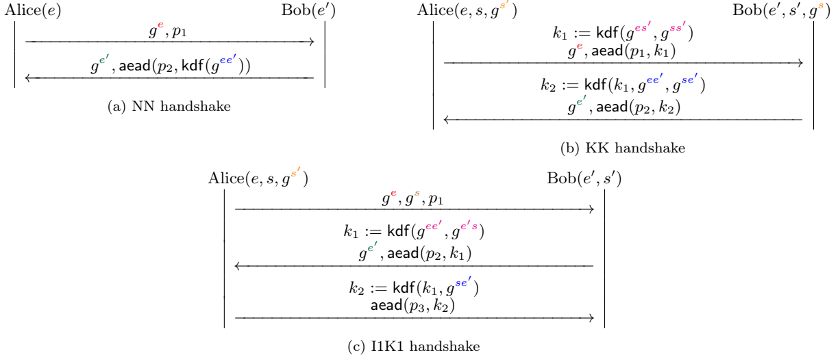
Figure 2: Alice & Bob notation for the handshakes of Figure 1. e, e' (respectively s, s' ) are ephemeral (respectively static) private keys and the p_i are payloads exchanged during the handshake. In transport mode, payloads are encrypted with the last key material used in the handshake. For legibility, we omitted the associated data of AEAD encryptions, which roughly corresponds to the hash of all preceding sent messages along with the public keys in pre-messages.
