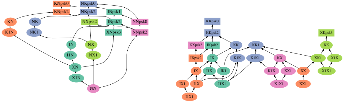
(a) Hierarchy of secrecy and agreement guarantees for protocols that do not require both the initiator and recipient having a static key. In this figure, we do not include anonymity properties to highlight the structure with only two maximal elements.
