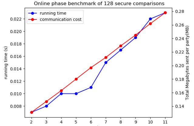
Figure 6. Online phase benchmark with different parameter settings ( n = 32, k is the number of blocks). The experiments are run using AWS t3.2xlarge instances with 130ms ping.
