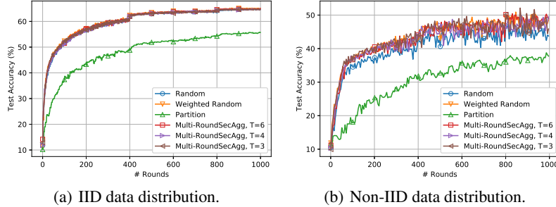
Figure 6: Training rounds versus test accuracy of LeNet in [23] on the CIFAR-10 with N = 120 and K = 12 . Key Metrics versus Test Accuracy. To investigate how the key metrics affect the test accuracy, we measure the test accuracy of the six schemes in the two settings, the IID and the non-IID settings. Our results are demonstrated in Figure 6. We make the following key observations.
