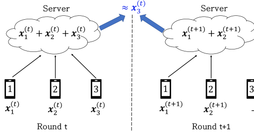
Figure 1: A multi-round secure aggregation example, where the server can reconstruct the model of user 3. At round t , the set of participating users is \mathcal{S}^{(t)} = \{1, 2, 3\} . At round t + 1 , the set of participating users is \mathcal{S}^{(t+1)} = \{1, 2\} . If the local models do not change significantly over the two rounds (e.g., the models start to converge), the server can reconstruct the model of user 3 from the aggregated models of the two rounds.
