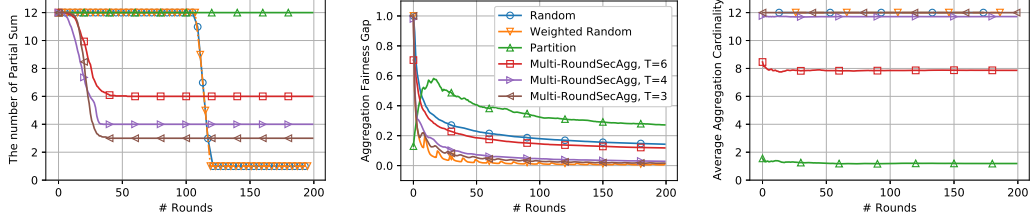
(a) Multi-round privacy guarantee. (b) Aggregation fairness gap. (c) Average aggregation cardinality. Figure 4: The key metrics with N = 120 (number of users), K = 12 (number of selected users at each round).
