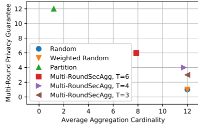
Figure 5: Trade-off between multi-round privacy guarantee versus average aggregation cardinality with N = 120 and K = 12 .
