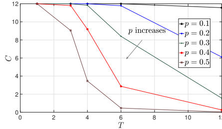
Figure 3: An illustration of the trade-off between the multi-round privacy guarantee T and the average aggregation cardinality C . In this example, N = 120 and K = 12 .
