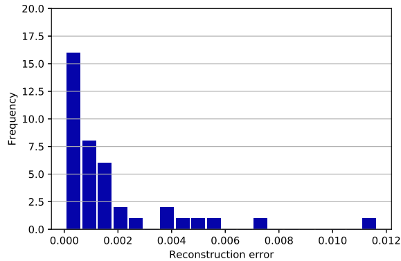
Figure 8: Histogram of the reconstruction error defined in (35) of N = 40 users when the K (= 8) -uniform random selection scheme is used to train the CNN [16] on the MNIST dataset.
