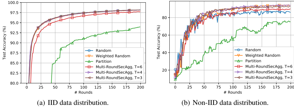
Figure 7: Training rounds versus test accuracy of CNN in [16] on the MNIST with N = 120 and K = 12 .
