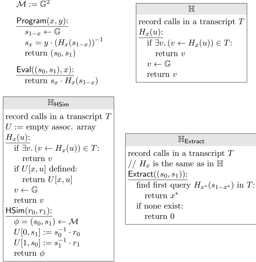
Figure 6: Batch 2-POPF based on the OT construction of Masny-Rindal [MR19]. Here H_0, H_1 : \mathbb{G} \rightarrow \mathbb{G} are random oracles, and (\mathbb{G}, \cdot) is a group.
