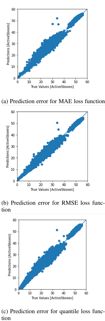
Fig. 4: Comparison of loss functions for baseline experiment (16-branch GFS)
