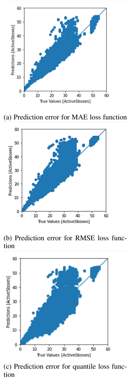
Fig. 5: Comparison of loss functions for generalization experiment (TWINE)
