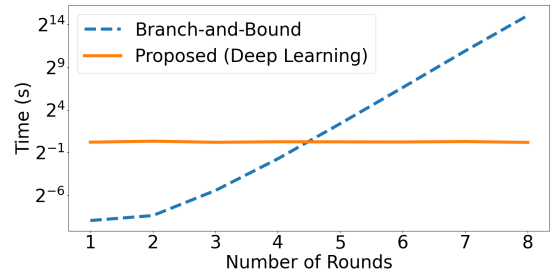
Fig. 6: Time required to label 10000 randomly selected truncated differential pairs
