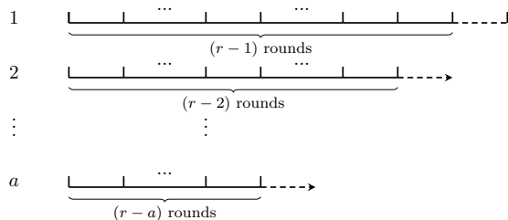
Figure 6: The deterministic differential characteristics embedded into LowMC-M.
