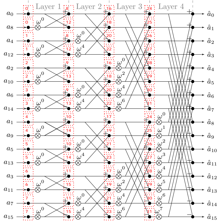
Figure 9: Example NTT_{br}^{CT} with n = 16 (unoptimized). In this case, one coefficient is stored in a single memory word, two coefficients can be loaded to the register file ( l = 2 ), and one pair of coefficients can be executed in parallel. The red boxes indicate which coefficients are stored together in one word (in this case they are not stored together) and in which order the coefficients are processed by a single butterfly unit.
