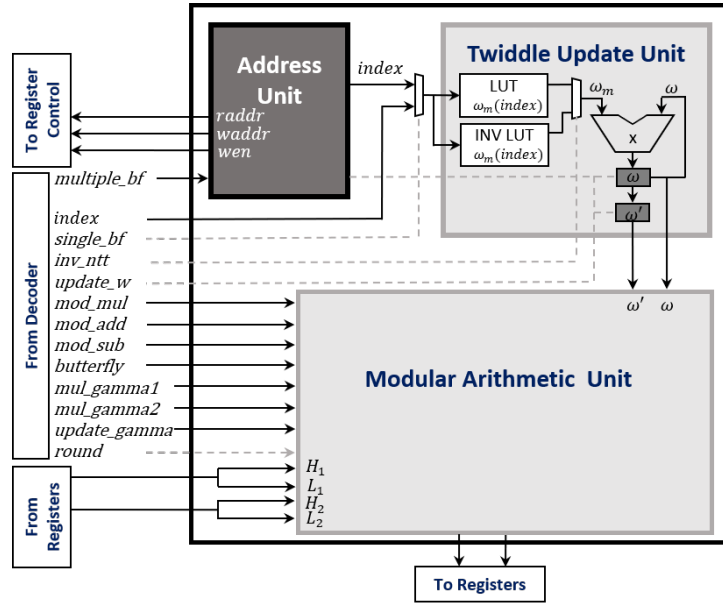
Figure 2: NTT and Modular Arithmetic Unit
