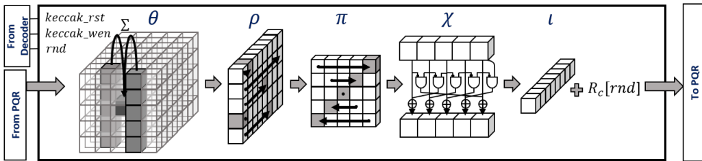
Figure 5: Keccak Accelerator
