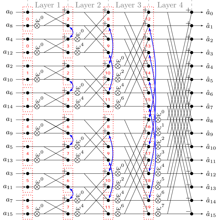
Figure 1: Example NTT_{br\ no}^{CT} with n = 16 . In this case, two coefficients are stored in a single word, eight coefficients can be loaded to the register file ( l = 8 ), and two pairs of coefficients can be executed in parallel. The red boxes indicate which coefficients are stored together in one word and in which order the coefficients are processed by the two butterfly units. The blue arrows show the coefficients which are swapped after the butterfly operations. For l = 8 , \log_2(l) - 1 = 2 layers were merged.
