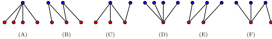
Fig. 3.3: Possible configuration of size = 4 edge subgraphs. Vertices in x^q are colored blue and vertices in u^q are colored red, and vertex labels are omitted for brevity.
