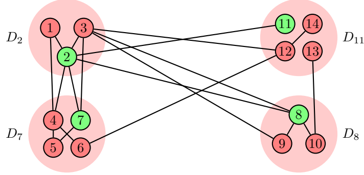
Figure 3: Extracting from 1-local adversarial sources using wedges. As before, a green node represents a good source and a red node represents a bad source. The red clouds D_2, D_7, D_8, D_{11} represent dependencies : cloud D_i contains all sources correlated with good source i . This placement of good sources and dependencies over our graph induces a cloud-wedge: (\{2, 7, 8\}, \{D_2, D_7, D_8\}) . The other good wedges do not induce cloud-wedges due to crossing edges in their terminal clouds.
