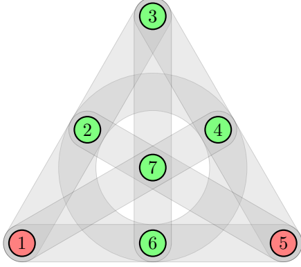
(a) The Fano plane , a 3-uniform hypergraph H = (V, \mathcal{E}) that is a Steiner triple system.
