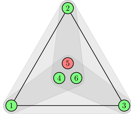
(b) A fragile set system H = (G, \mathcal{S}) , with \mathcal{S} = \{\{1, 2, 4, 5, 6\}, \{2, 3, 4, 5, 6\}, \{1, 3, 4, 5, 6\}\} .
