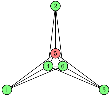
(a) A graph G = (V, E) that contains many wedges.
