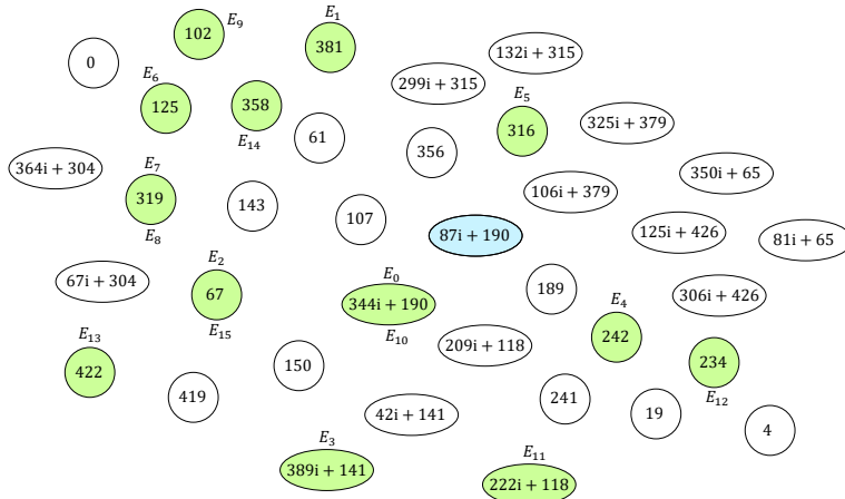
Fig. 11. Alice’s possible destination nodes (in green) when starting at E with j(E) = 87i + 190 , and computing 2^4 -isogenies to the curves E_k = E / \langle P_A + [k]Q_A \rangle with k \in \{0, 1, \dots, 15\} .
