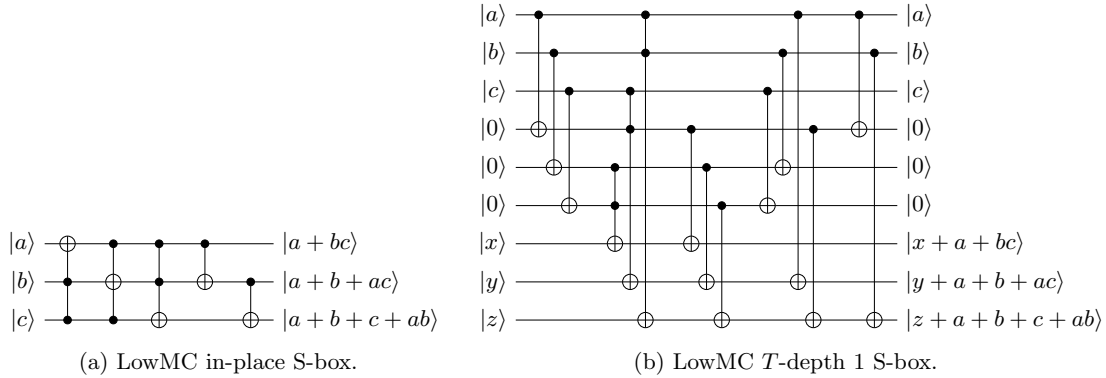
Fig. 5: Alternative quantum circuit designs for the LowMC S-box. The in-place design requires auxiliary qubits as part of the concrete CCNOT implementation.
