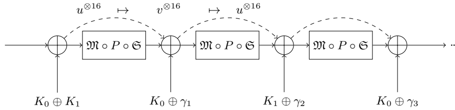
Fig. 2. If u \neq v , this figure depicts an invariant for two rounds which is not invariant under one round.
