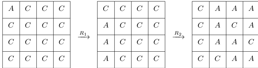
Fig. 9. Integral property for two rounds of MANTIS.
