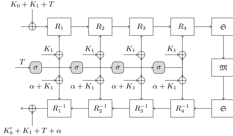
Fig. 7. Overview of MANTIS-4.
