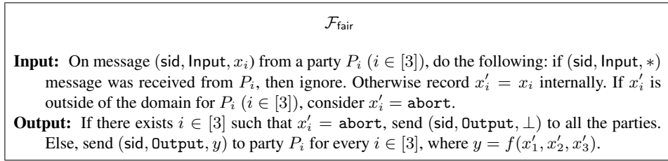
Fig. 12: Ideal Functionality for fairness
