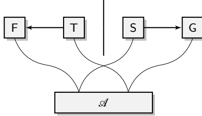
Fig. 2.1: Indistinguishability Game
