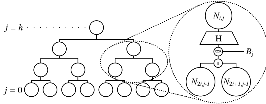
Fig. 2. The XMSS tree construction
