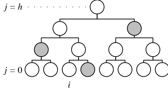
Fig. 1. The authentication path for a leaf i .
