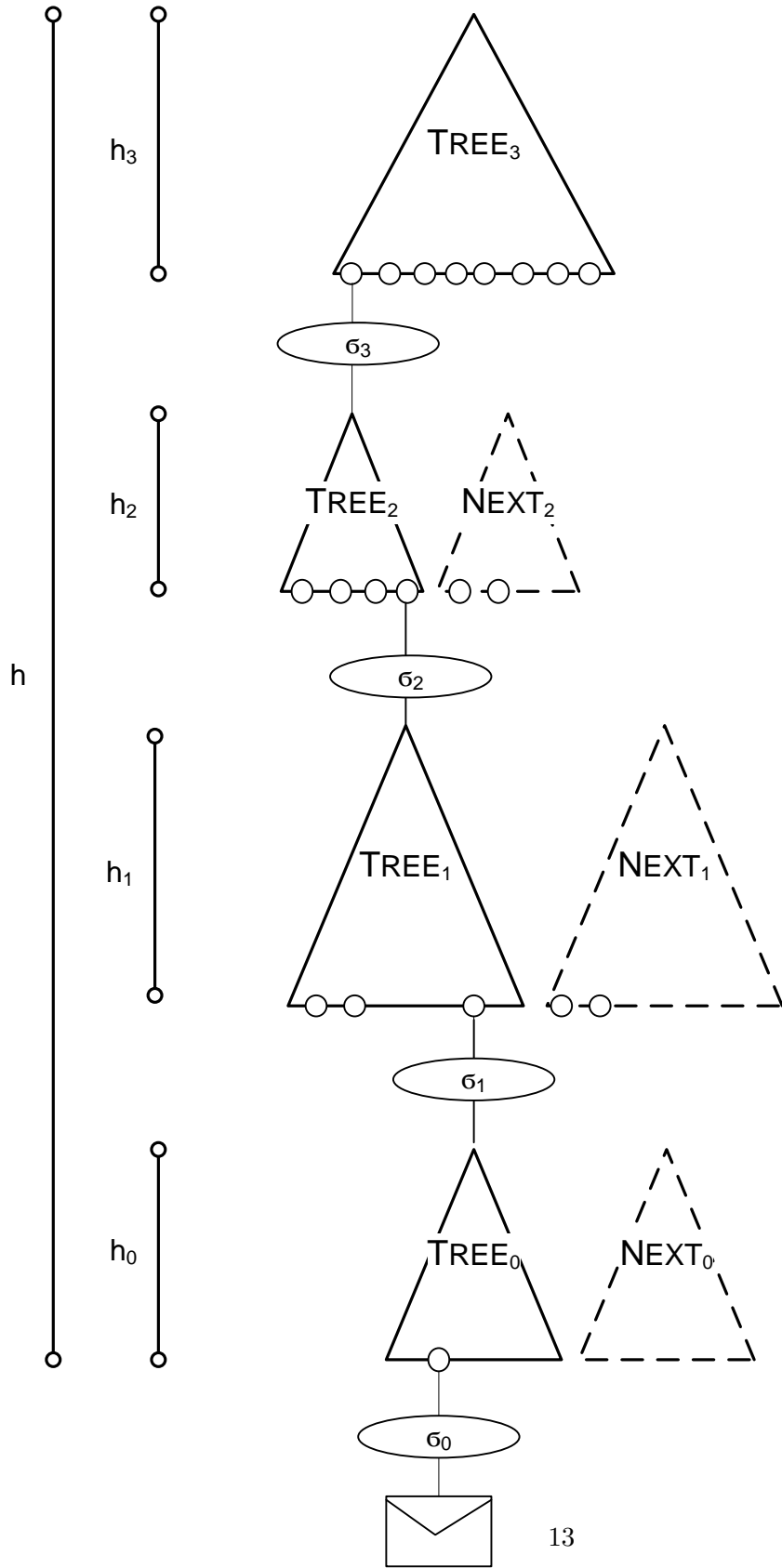
Fig. 3. A schematic representation of a XMSS MT instance with four layers
