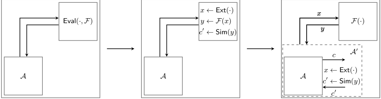
Figure 1. Oblivious reduction part 1 of 2.
