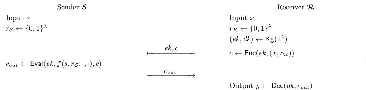
Figure 3. Oblivious Two-Party Protocol
