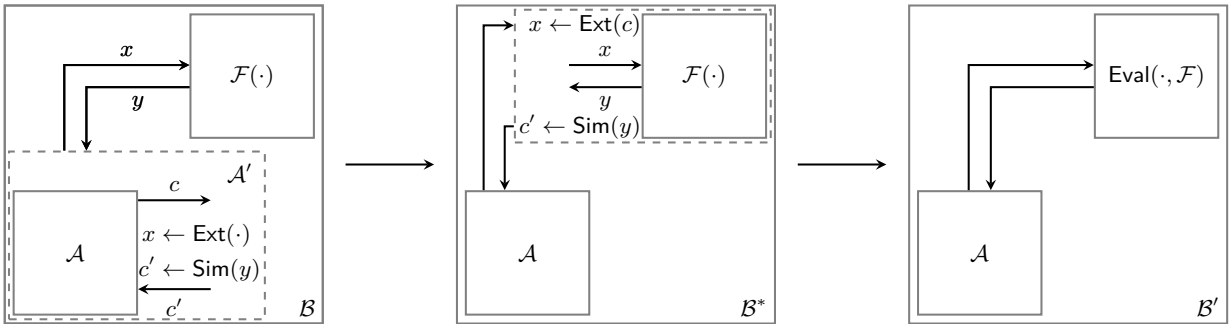
Figure 2. Oblivious reduction part 2 of 2.
