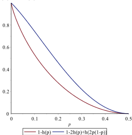
Fig. 3. Capacity of the original binary symmetric channel vs. capacity of the channel model corresponding to the probability computations (7) and (8).
