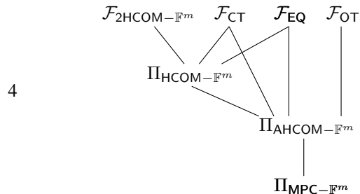
Fig. 4. Outline of functionalities and protocols
