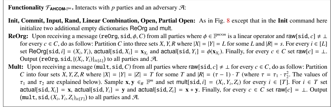
Fig. 11. Ideal Functionality \mathcal{F}_{\text{AHCOM-}\mathbb{F}^m}
