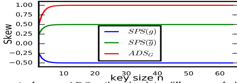
Fig. 9. Impact of n on ADS_G , the absolute difference of skew at the inputs of gate G , the output of Anti-SAT block, for p = 1 . SPS(g) and SPS(\bar{g}) represent the skew of the AND and NAND tree in the Anti-SAT block.
