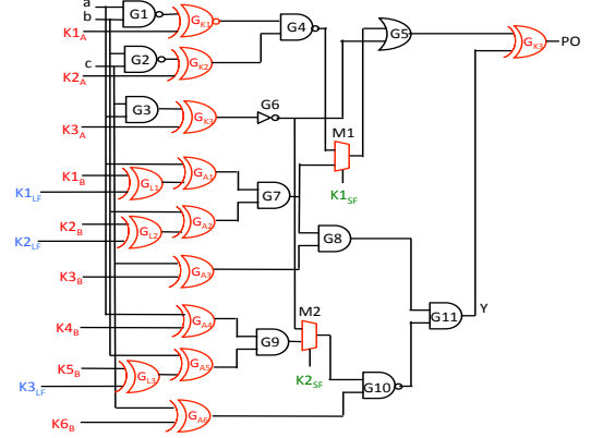
Fig. 7. Functional and structural obfuscation between Anti-SAT and logic locked circuit of Figure 2(c). \{K_{1A}, \dots, K_{3A}\} are the key inputs to the logic locked circuit, \{K_{1B}, \dots, K_{6B}\} are the key inputs to the Anti-SAT circuit, \{K_{1LF}, \dots, K_{3LF}\} (blue) are the key inputs for functional obfuscation, and \{K_{1SF}, K_{2SF}\} (green) are the key inputs for structural obfuscation. M1 and M2 are used for MUX-based logic locking.
