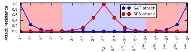
Fig. 10. Normalized attack resistance of the Anti-SAT block for n = 16 . For the SAT attack, the resistance is the number of iterations of the attack normalized by 65536. For the SPS attack, the resistance is specified as 1 - ADS_G . The SPS attack is highly effective in region shaded red; the SAT attack is effective in the region shaded blue.
