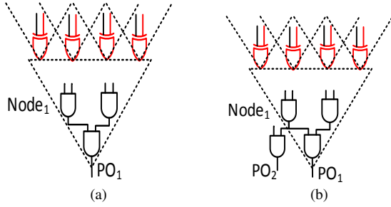
Fig. 13. a) A non-decomposable AND tree, and b) a decomposable AND-tree [27]. Attacks on the decomposable tree can leverage divide-and-conquer strategies.
