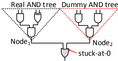
Fig. 14. Insertion of dummy AND-tree in the circuit. A stuck-at-0 fault is introduced at the dummy input of the OR gate [27].
