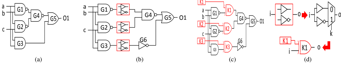
Fig. 2. (a) The original circuit. (b) A camouflaged circuit consisting of INV/BUF camouflaged gates. (c) Equivalent logic locked circuit constructed by replacing INV/BUF camouflaged gates with XOR key gates. (d) Transforming an INV/BUF camouflaged to its logic locking counterpart using a MUX; further simplification of the MUX-based gate to an XOR key gate [19].
