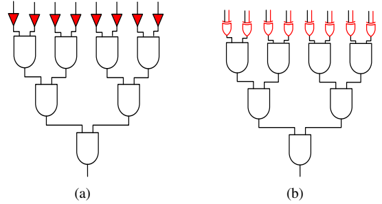
Fig. 12. Examples of AND/OR-tree insertion: a) A camouflaged AND-tree with camouflaged INV/BUF gates inserted at its inputs [27], b) The locked counterpart of the AND-tree with XOR/XNOR key gates inserted at its inputs, using the transformations in [19]. Both trees achieve the same level of security against the SAT attack [17], [24].
