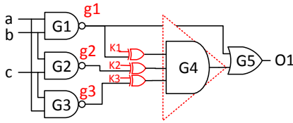
Fig. 17. An example of pruned input pattern space as identified by the sensitization stage. The locked AND tree G4 has three inputs: g1, g2, and g3. The TFI logic prevents the tree inputs from taking on the values 001, 010, and 101. The TFO logic further reduces the number of feasible inputs; overall, only two out of eight possible input combinations, 011 and 000, are feasible for the AND tree inputs.
