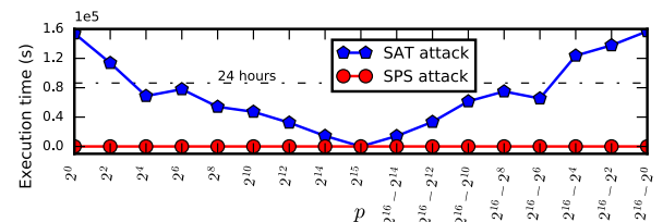
Fig. 11. Execution time of the SAT attack and the SPS attack on basic Anti-SAT block for n = 16 . The execution time of the SAT attack is more than a day for p \in \{1, 2^n - 1\} , whereas, the execution time of the SPS attack is less than 2 minutes for all values of p .
