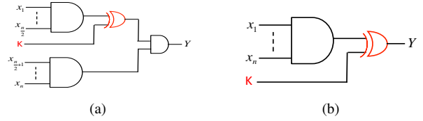
Fig. 8. (a) Key gate inserted inside the tree of n -input AND gate; the change in probability skew assists the SPS attack. (b) Key gate inserted at the output of n -input AND gate assists the SAT attack [24].
