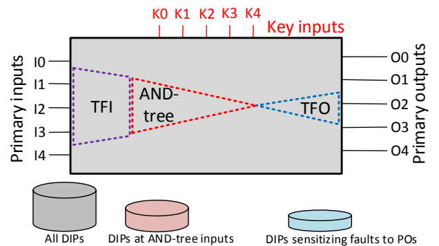
Fig. 16. An illustration of how the sensitization stage reduces the number of the required DIPs. The gates in the TFI of the tree introduce bias and reduce the number of patterns received at the tree inputs. The gates in the TFO hamper the sensitization of errors activated at the output of the AND tree and further narrow down the attack pattern space.
