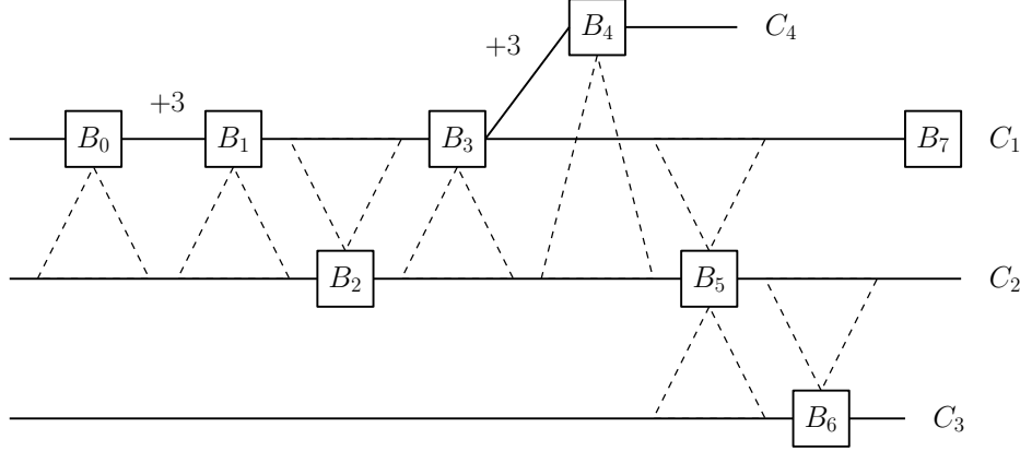
Figure 4: An example of the matching described in the claim in Lemma 18. B_0, \dots, B_7 are u.s. blocks and the dashed triangles point to the places where according to Lemma 16 there should exist an adversarial block. In this example we can use Lemma 16 two times for block B_5 . The “extra” block is matched to B_7 .
