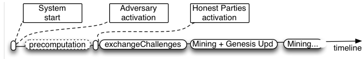
Figure 1: Timeline and phases of the bootstrapped Bitcoin backbone protocol.
