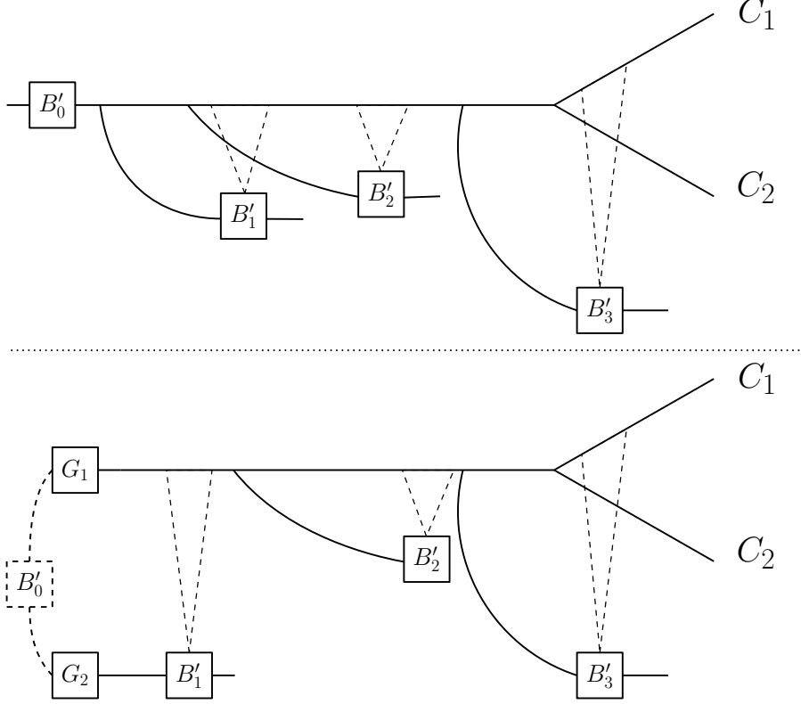
Figure 5: An example of two scenarios for the matching described by Lemma 18. Notice that in the second one an artificial block B'_0 has been introduced to aid our analysis.
