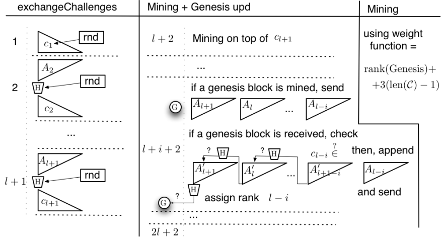
Figure 2: The different phases of the bootstrapped backbone protocol.
