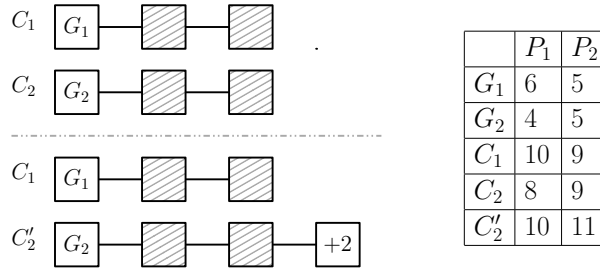
Figure 3: An example where blocks weigh 2 units. In the table the weights of the respective chains are depicted. Initially player P_1 has adopted chain C_1 and player P_2 chain C_2 . Then a uniquely successful round happens and C_2 is extended to C_2' . Notice that, P_1 will not adopt C_2' since it has the same weight as C_1 . If the new block weighted 3 units, all players would have adopted chain C_2' .
