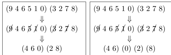
Fig. 1. Example of how one round of reverse 2-cycle walking differs from regular cycle walking. In this example, \mathcal{T} = \{0, \dots, 9\} and \mathcal{S} are the even numbers in \mathcal{T} . Left: the effect regular cycle walking has on the cycle structure of the permutation. Right: the effect of one round of reverse 2-cycle walking on the cycle structure.
