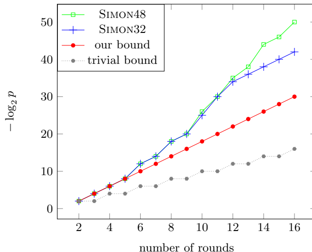
Fig. 1. Comparison of the experimental bounds for SIMON32 and SIMON48 as described in [21, Section 5.2] and our provable bounds.
