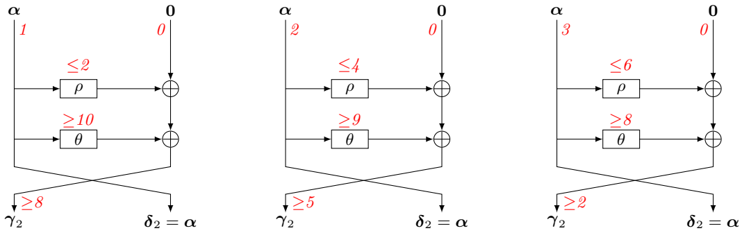
Fig. 3. Propagation of the differential Hamming weight for \text{wt}(\alpha) \in \{1, 2, 3\} .
