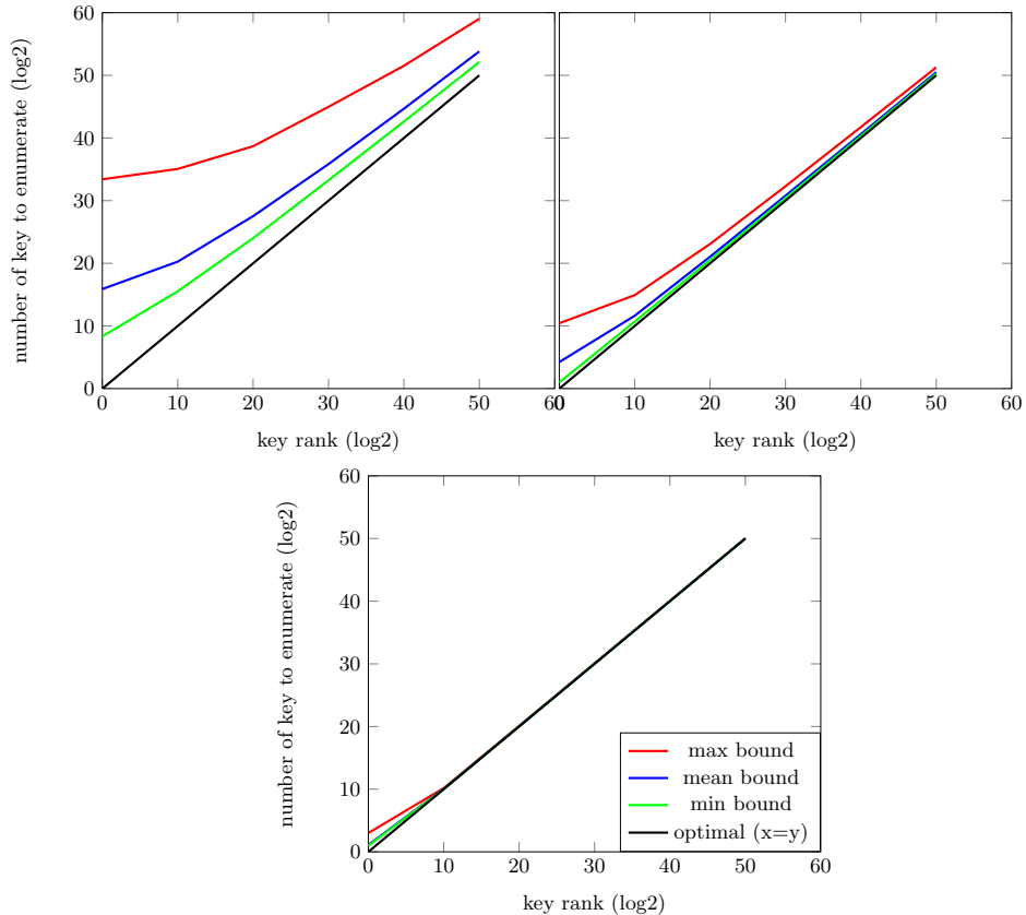
Fig. 4. Enumeration overheads due to rounding errors with \text{merge}_1 (i.e. no merging). Upper left: 256 bins. Upper right: 2048 bins. Bottom: 65536 bins.
