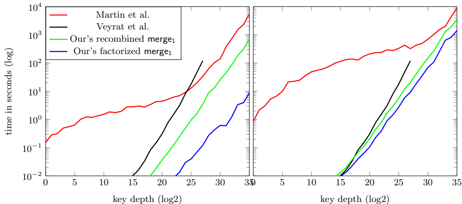
Fig. 7. Execution time for the java implementation of Veyrat et al., Martin et al. and ours with 8 bits of precision (left) and 11 bits of precision (right).
