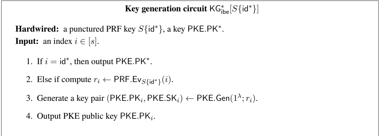
Figure 4: Circuit \text{KG}_{\text{ibe}}^*[S\{\text{id}^*\}]
