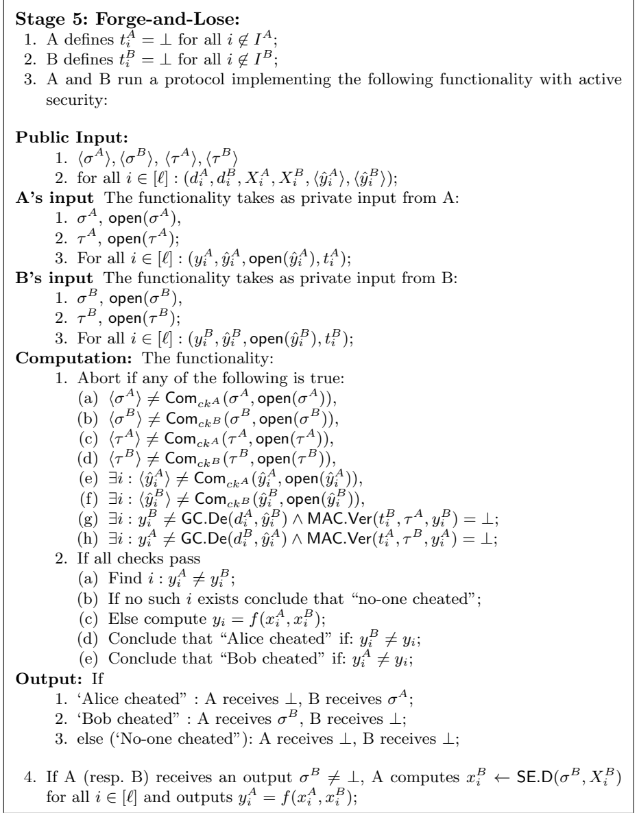
Figure 5. Stage 5: Forge-and-Lose
