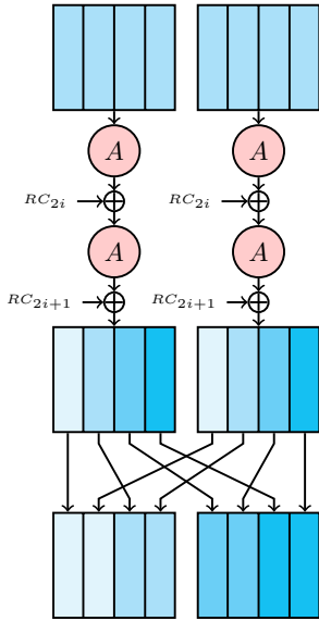
Figure 3: Haraka-256/256 step function.
