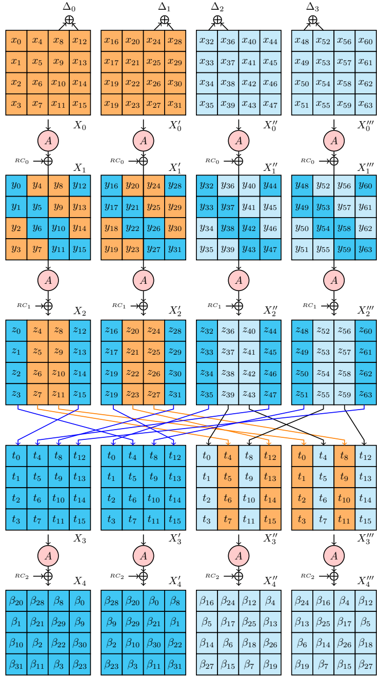
Figure 7: General overview of the final phase of the preimage attack. the dark blue bytes are guessed and the orange bytes are deduced.
