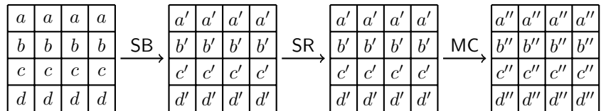
Figure 5: An AES state with four equal columns is called strongly symmetric, and stays strongly symmetric after the application of (any number of) the keyless AES round function.
