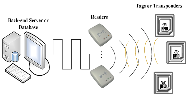
Fig. 1. An RFID system architecture.
