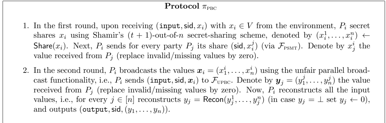
Figure 10: The parallel broadcast protocol, in the (\mathcal{F}_{\text{PSMT}}, \mathcal{F}_{\text{UPBC}}) -hybrid model
