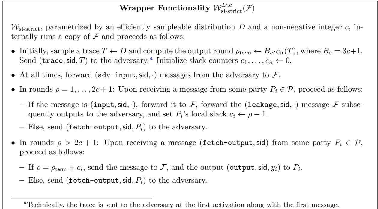
Figure 6: The slack-tolerant strict wrapper functionality
