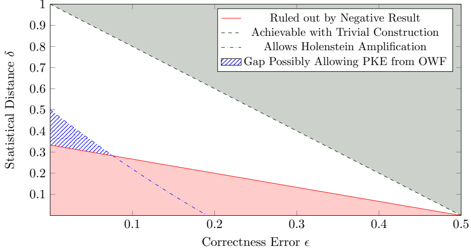
Figure 1: The graph gives an overview over the possible range of parameters for \text{saiO} . In the upper right are parameter regimes that can be achieved using the construction described in Appendix A. In the lower left are the strong parameter regimes ruled out by our negative result in Section 3. The graph shows nicely the gap between the parameters that can be ruled out and those that can be used to construct public key encryption using the construction of Sahai and Waters as well as the amplification technique of Holenstein.
