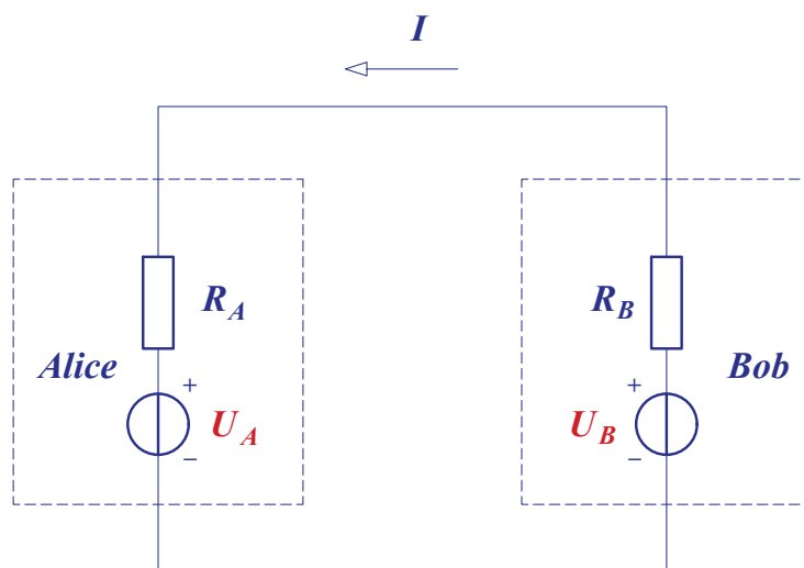
FIGURE 1. Electrical circuit
