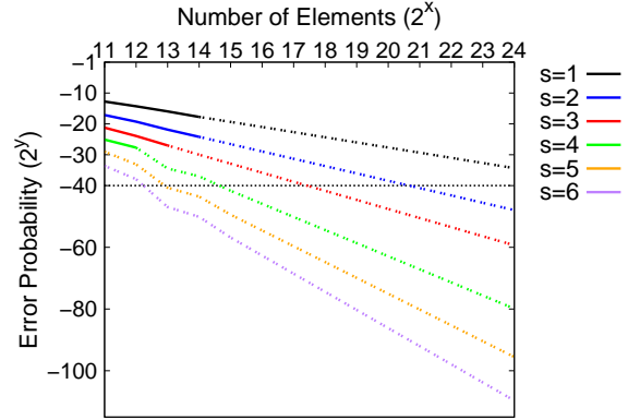
Figure 2: Error probability when mapping n elements to 2.4n bins using 2-way Cuckoo hashing for stash sizes 1 \leq s \leq 6 . The solid lines correspond to actual measurements, the dashed lines were extrapolated using linear regression. Both axes are in logarithmic scale.
