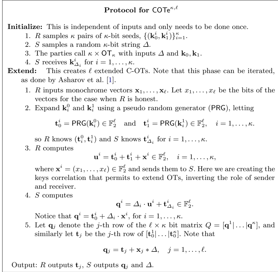
Fig. 3. Protocol for correlated OT with errors between S and R .
