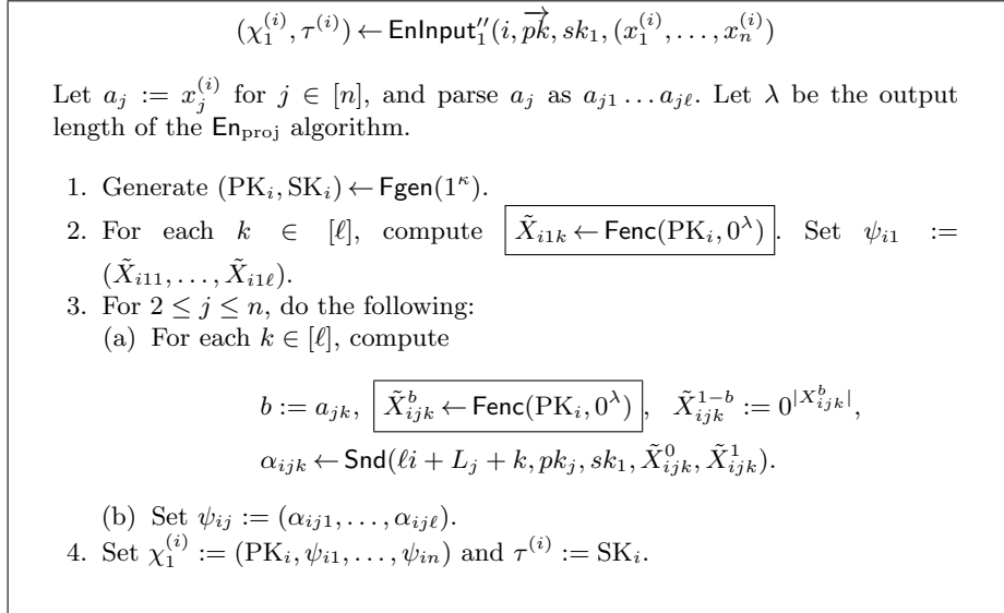
Fig. 3. Description of \text{EnInput}''_1
