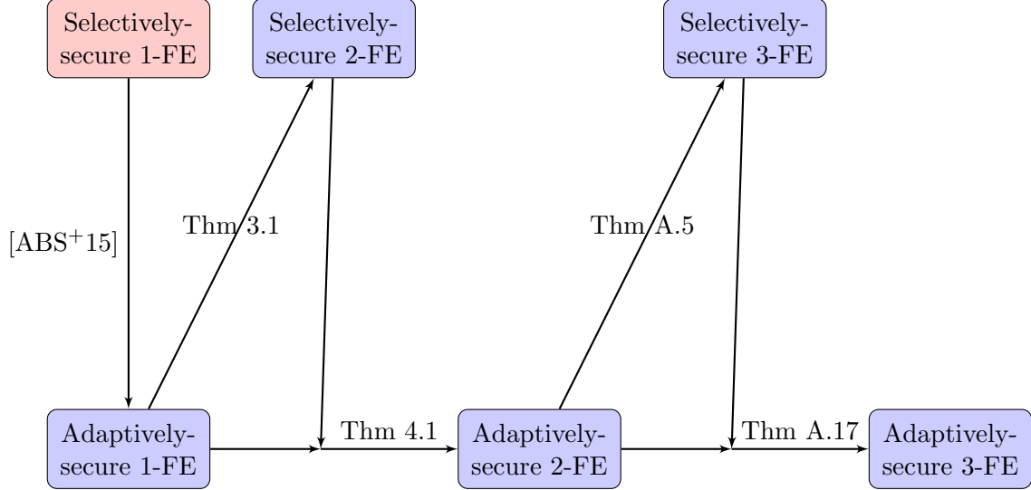
Figure 1: An illustration of the required iterative applications of our two transformations for obtaining an adaptively-secure three-input scheme based on any selectively-secure single-input scheme.
