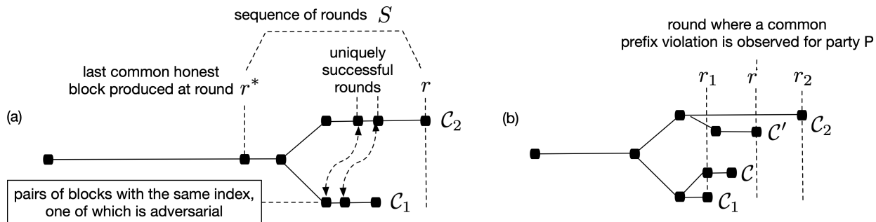
Figure 3: Illustration of proofs of Lemma 14 and Theorem 15.
