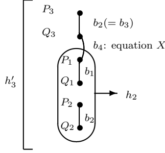
Figure 3: Computation of h'_3 from h_2 on this example.
