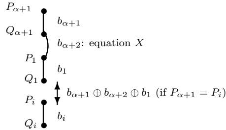
Figure 1: “6-point figure” for X + (1 \text{ equation } P_{\alpha+1} = P_i) .
