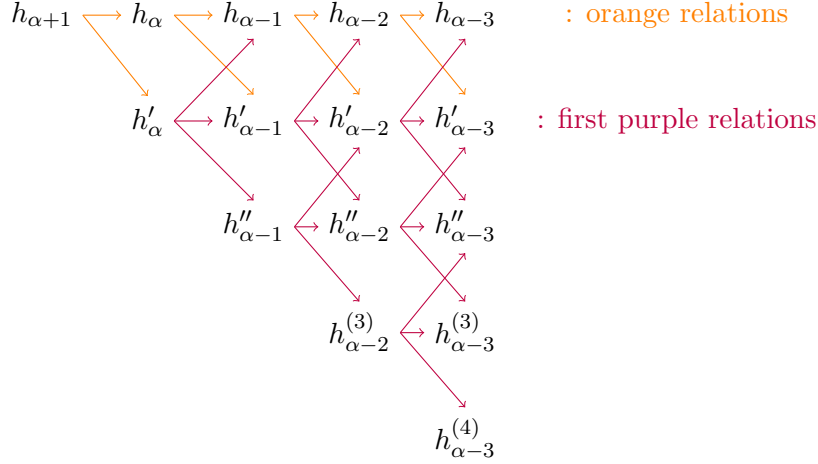
Figure 5: General view of the “colored proof strategy” used in this paper
