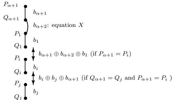
Figure 2: “8-point figure” for X + 2 equations
