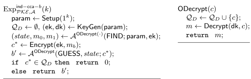
Figure 3: \mathcal{PK}\mathcal{E} : Semantic Security against Chosen-Ciphertext Attacks (IND-CCA)
