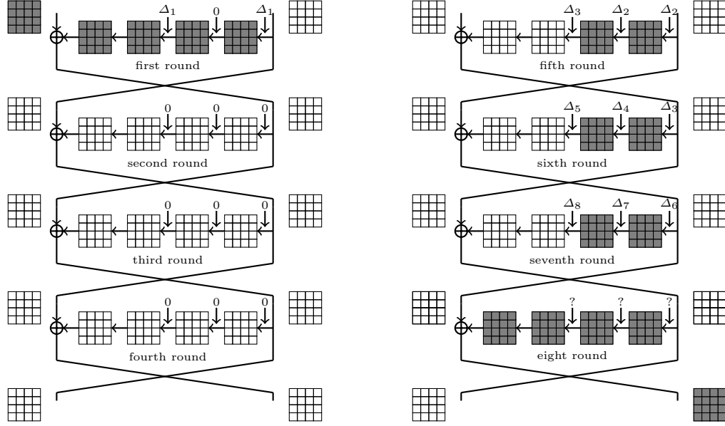
Fig. 5. The 8-round truncated differential path. The left part represents the four first rounds and the right part the four last ones. Each gray cell stands for an active byte. The \Delta 's in each round denote the differences incorporated by the subkeys. For the 7-round differential path, we remove the differences control in the seventh round.
