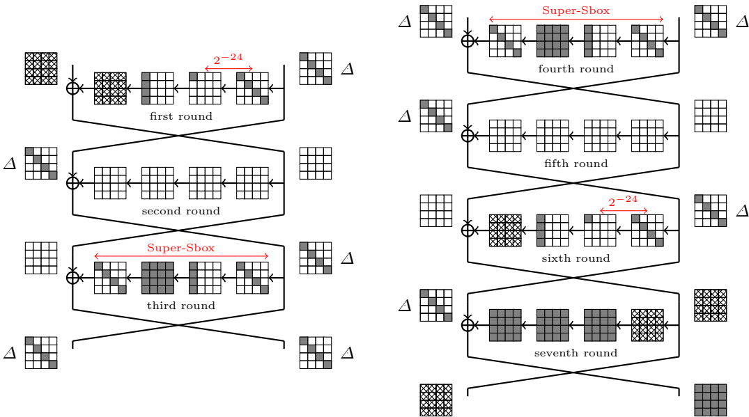
Fig. 4. The 7-round truncated differential path. The left part represents the three first rounds and the right part the four last ones. Each gray cell stands for an active byte. A hatched state denotes a fully active state obtained by applying the MixColumns function on only one active byte per column. During the path, all D 128-bit words contain the difference \Delta .
