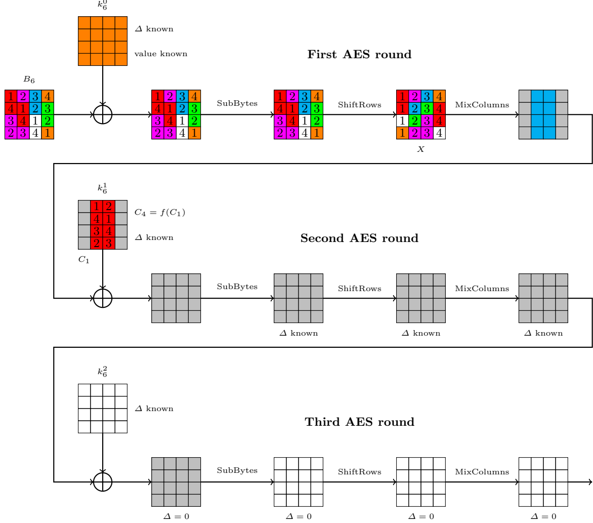
Fig. 8. The 3 AES rounds of the seventh round: the red bytes will determine the middle columns of k_6^1 (because of the message expansion and of previous conditions); the blue bytes will determine the differences in the 2 middle columns on the input of the second round; the orange bytes are fixed (due to round 6); the white and light gray bytes are free. The green bytes are the results of an XOR between blue bytes and orange bytes whereas pink bytes are the results of an XOR between blue bytes and red bytes.
