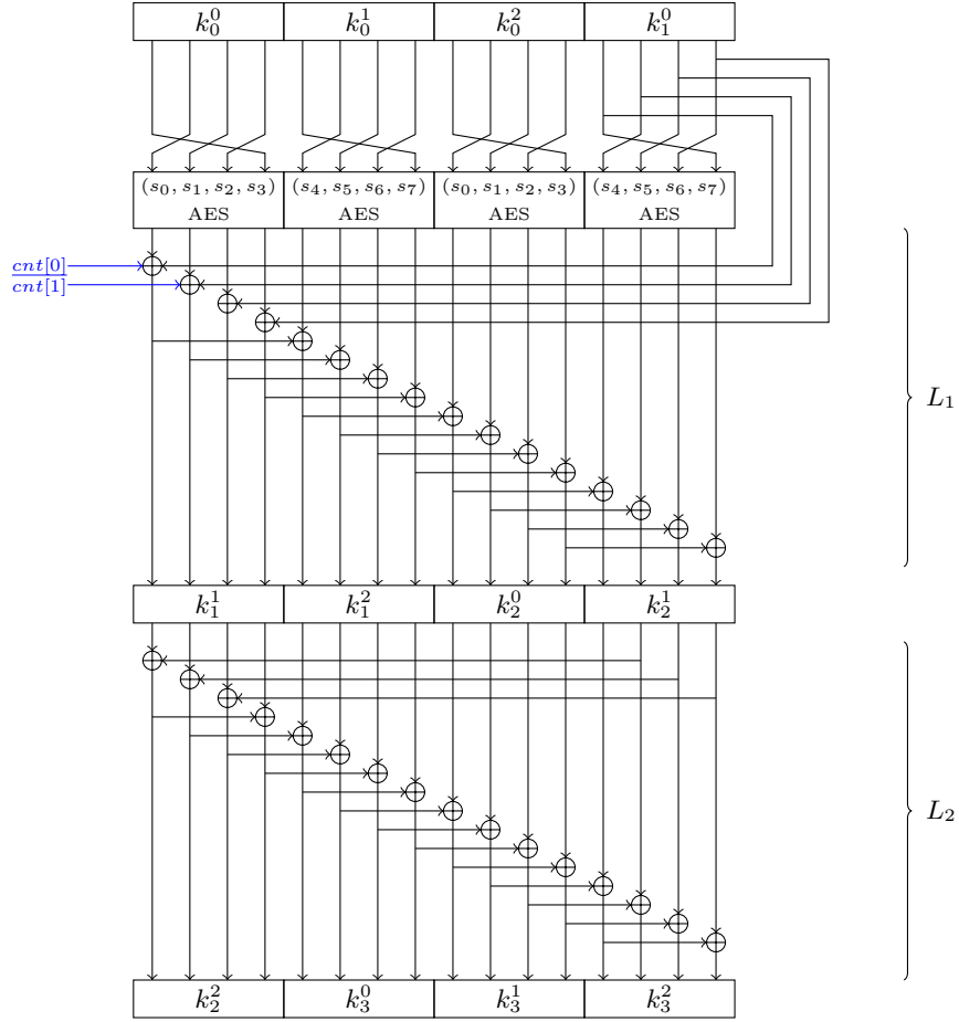
Fig. 2. The first step of the message expansion of the SHAvite-3-256 compression function. Note that the salt words are XORed to the internal state before the parallel AES rounds application. Moreover, the counters are XORed in different positions for different steps of the message expansion.
