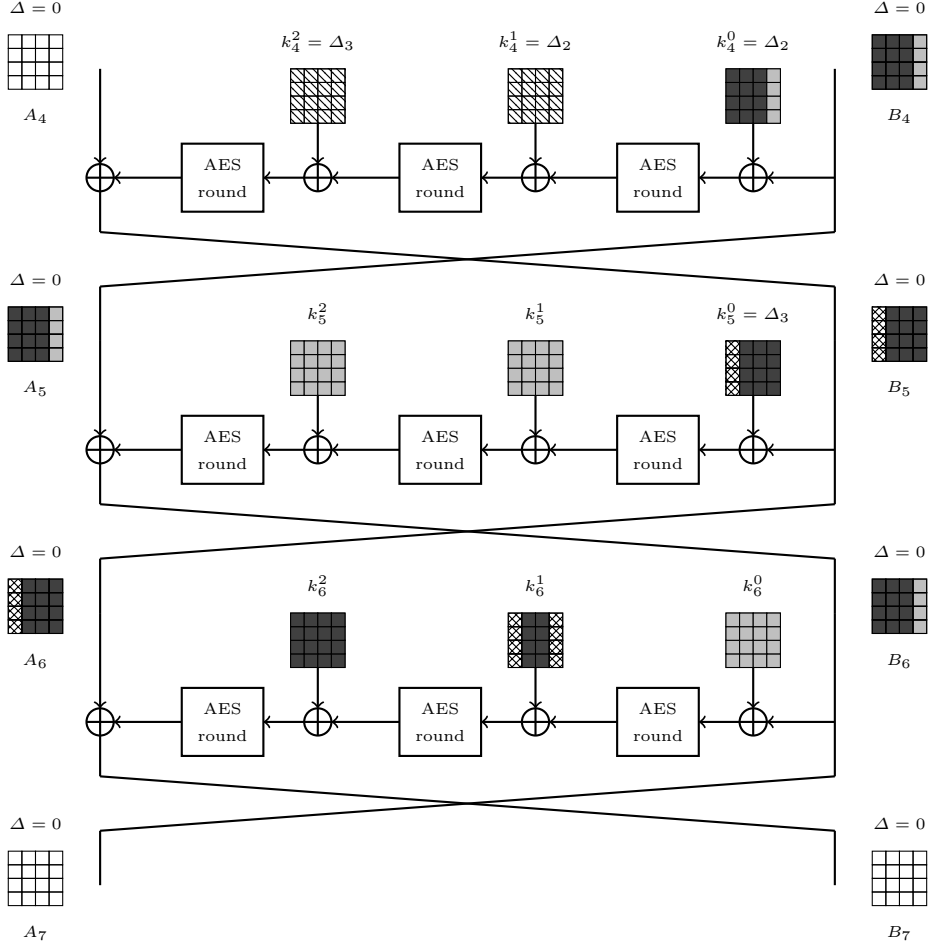
Fig. 7. Details of rounds 5, 6 and 7 of the 8-round chosen-related-salt distinguisher on the SHAvite-3-256 compression function. The bytes denoted with north-west lines are fixed during the fifth round. The light gray bytes are fixed during the sixth round. The dark gray bytes are fixed at the beginning of the seventh round whereas the bytes denoted with hatched cells are fixed at the end of the seventh round.
