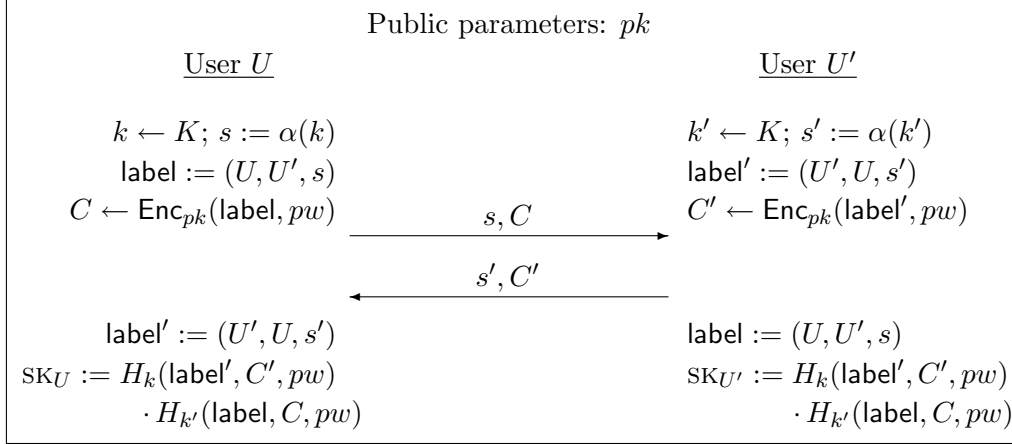
Figure 1: A one-round protocol for password-based authenticated key exchange.
