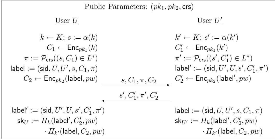
Figure 2: A universally composable protocol for password-based authenticated key exchange.
