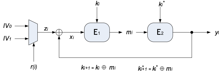
Fig. 7. Secure initialization of the PRNG.
