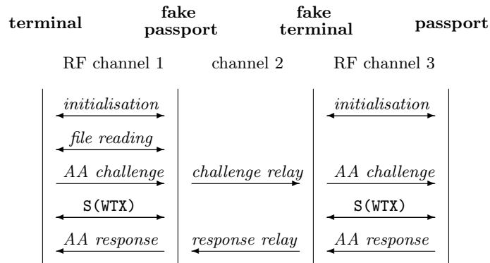
Fig. 1. Relay attack on active authentication (AA)
