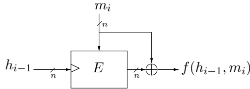
Figure 1: The Matyas-Meyer-Oseas (MMO) compression function [13], called H_1 in [3]. E: \{0, 1\}^n \times \{0, 1\}^n \rightarrow \{0, 1\}^n is a block cipher; the hatch mark denotes the location of the key. Iterating this compression function results in a provably-secure blockcipher-based hash function in the ideal-cipher model.
