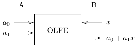
Fig. 3. Oblivious linear-function evaluation over GF(q) .
