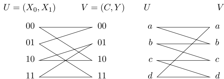
Fig. 2. Left hand side: The distribution of \binom{2}{1} -OK. (Each edge is a possible combination with probability 1/8 .) Right hand side: The distribution arising from the “noisy-typewriter channel.” Obviously, the two distributions are equivalent.
