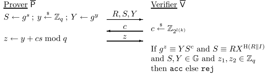
Figure 19: The \mathcal{BAN} -IBI scheme. The scheme is parameterized by super-logarithmic challenge length l : \mathbb{N} \rightarrow \mathbb{N} , a random oracle \text{H} : \{0, 1\}^* \rightarrow \{0, 1\}^{\ell(k)} and a prime-order cyclic group generator \text{K}_{\text{cg}} such that 2^{l(k)} < q for all (\langle \mathbb{G} \rangle, q, g) \in [\text{K}_{\text{cg}}(1^k)] . The prover \bar{\text{P}} and verifier \bar{\text{V}} are run on initial states usk = (\langle \mathbb{G} \rangle, q, g, R, s) and (mpk, I) where mpk = (1^k, \langle \mathbb{G} \rangle, q, g, X) , respectively.
