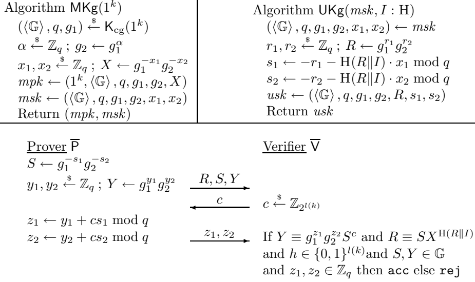
Figure 16: The \text{OKDL-IBI} scheme. The scheme is parameterized by super-logarithmic challenge length l : \mathbb{N} \rightarrow \mathbb{N} , a random oracle \text{H} : \{0, 1\}^* \rightarrow 0, 1^{l(k)} and a prime-order cyclic group generator \text{K}_{\text{cg}} such that 2^{l(k)} < q for all (\langle\mathbb{G}\rangle, q, g) \in [\text{K}_{\text{cg}}(1^k)] . The prover \bar{\text{P}} and verifier \bar{\text{V}} are run on initial states \text{usk} = (\langle\mathbb{G}\rangle, q, g_1, g_2, R, s_1, s_2) and (\text{mpk}, I) where \text{mpk} = (1^k, \langle\mathbb{G}\rangle, q, g_1, g_2, X) , respectively.
