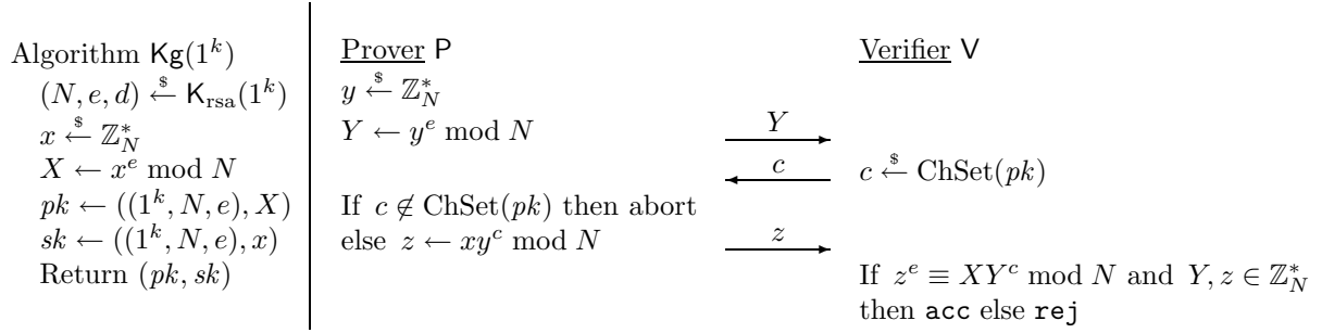
Figure 10: The \mathcal{S}\mathcal{h} -SI and \mathcal{S}\mathcal{h}^* -SI schemes. Both schemes are specified in terms of a prime-exponent RSA generator \mathsf{K}_{\text{rsa}} and super-logarithmic challenge length l(\cdot) such that 2^{l(k)} < e for all (N, e, d) \in [\mathsf{K}_{\text{rsa}}(1^k)] . The prover P and verifier V are initialized with states sk = ((1^k, N, e), x) and pk = ((1^k, N, e), X) , respectively. The \mathcal{S}\mathcal{h} -SI and \mathcal{S}\mathcal{h}^* -SI differ from each other in that the former uses challenge set \text{ChSet}(pk) = \{0, \dots, 2^{l(k)} - 1\} , while the latter uses \text{ChSet}(pk) = \{1, \dots, 2^{l(k)}\} .
