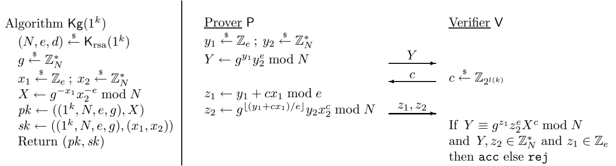
Figure 11: The \text{OkRSA-SI} scheme. The scheme is parameterized with a prime-exponent RSA generator \text{K}_{\text{rsa}} and a challenge length l : \mathbb{N} \rightarrow \mathbb{N} such that 2^{l(k)} < e for any e output by \text{K}_{\text{rsa}}(1^k) . The prover P and verifier V are initialized with states sk = ((1^k, N, e, g), (x_1, x_2)) and pk = ((1^k, N, e, g), X) , respectively.
