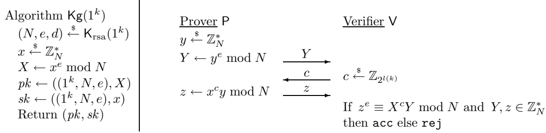
Figure 9: The \mathcal{GQ}\text{-SI} scheme. The scheme is parameterized with a prime-exponent RSA key generator \text{K}_{\text{rsa}} and a superlogarithmic challenge length l: \mathbb{N} \rightarrow \mathbb{N} such that 2^{l(k)} < e for all (N, e, d) \in [\text{K}_{\text{rsa}}(1^k)] . The prover \text{P} and verifier \text{V} are initialized with states sk = ((1^k, N, e), x) and pk = ((1^k, N, e), X) , respectively.
