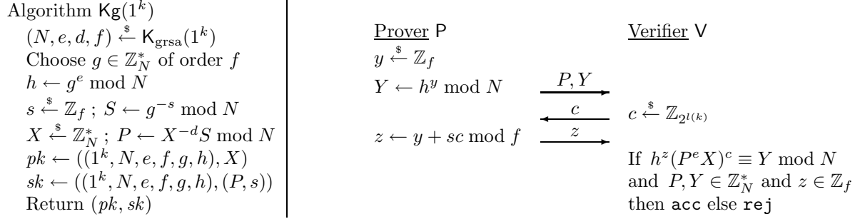
Figure 12: The Gir-SI scheme. The scheme is parameterized with a challenge length l(k) and a Girault-RSA key generator \text{K}_{\text{grsa}} . The prover \text{P} and verifier \text{V} are initialized with states sk = ((1^k, N, e, f, g, h), (P, s)) and pk = ((1^k, N, e, f, g, h), X) , respectively.
