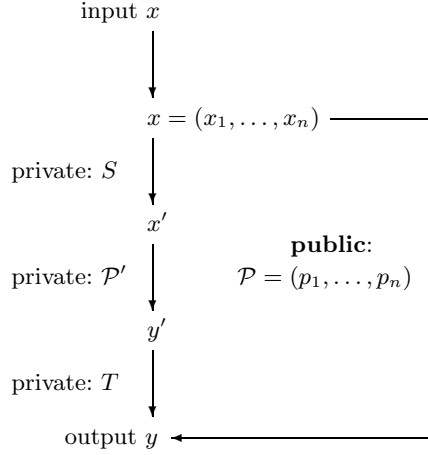
Fig. 2. \mathcal{MQ} -trapdoor (S, P', T) in STS
