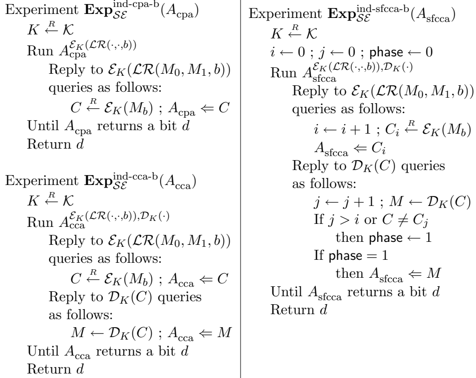
Figure 2: Experiments for Definition 6.2.
