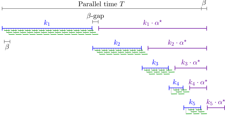
Figure 1: The “compute” and “proof” phases for each of m sub-computations. The i th sub-computation consists of k_i steps, while pipelining updates which each take \beta time. After finishing all updates, the prover computes the proof which takes k_i \cdot \alpha^* time.
