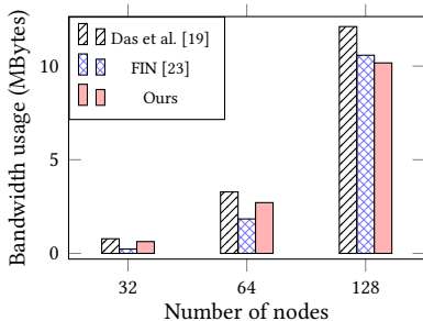
Figure 1: Bandwidth usage
