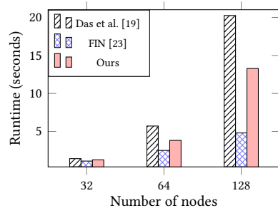
Figure 3: Runtime
