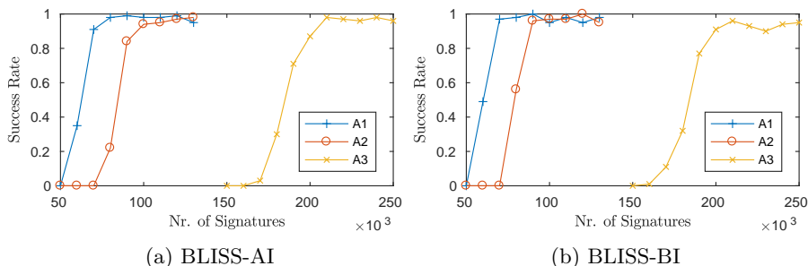
Fig. 1. Success rate of LPN decoding for the attack on shuffling
