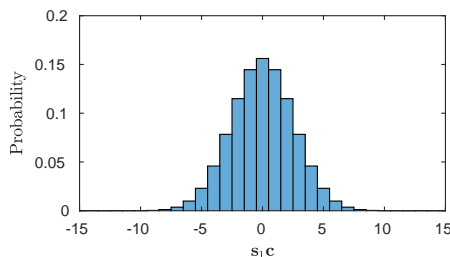
Fig. 4. Coefficient-wise probability distribution of \mathbf{s}_1 \cdot \mathbf{c}'
