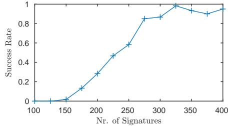
Fig. 2. Success rate of LPN decoding for an idealized attack on CDT sampling
