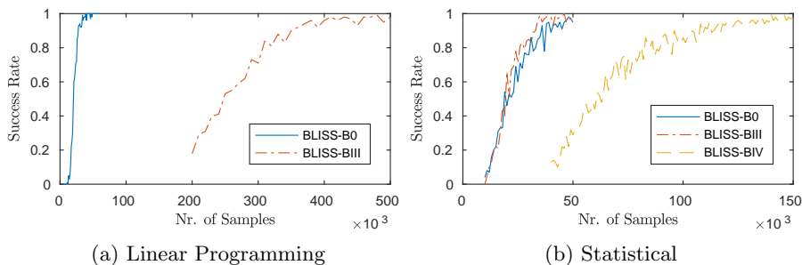
Fig. 3. Success rate for Twos recovery
